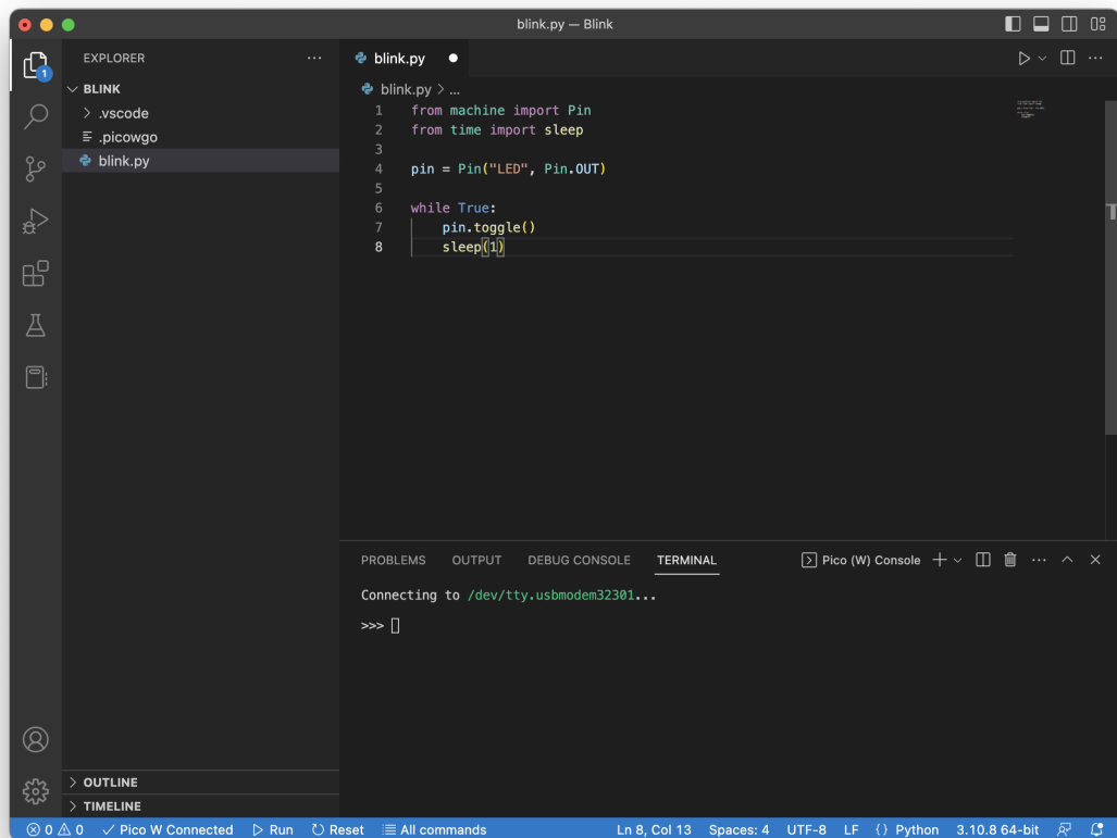
Figure 8. Visual Studio Code running with the Pico-W-Go extension connected to a Raspberry Pi Pico 2.
